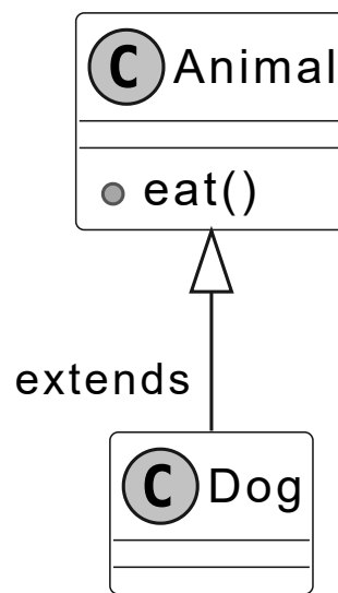
Single inheritance
