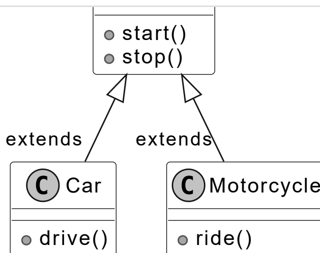
Hierarchical inheritance
