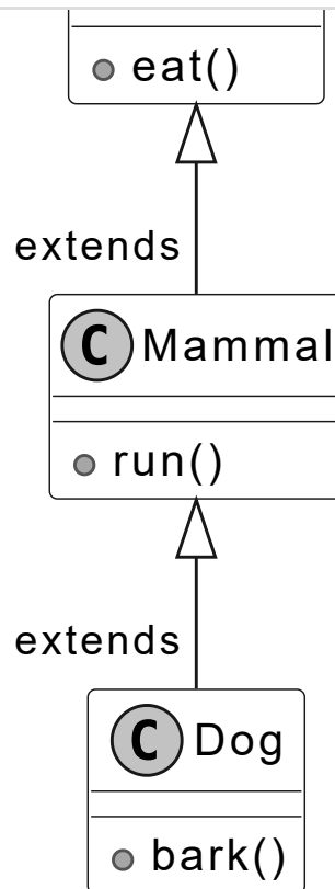
Multilevel inheritance
