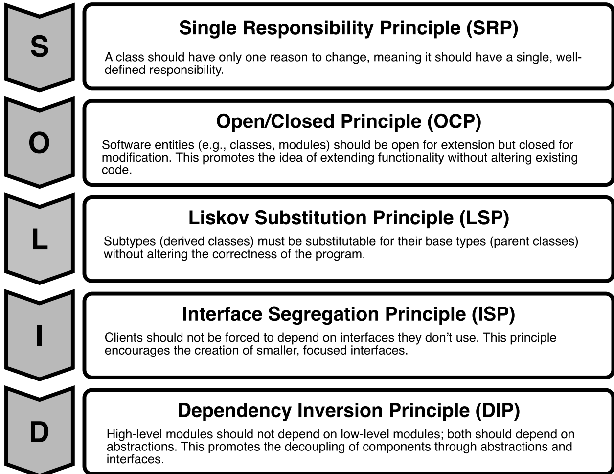
SOLID Principles
